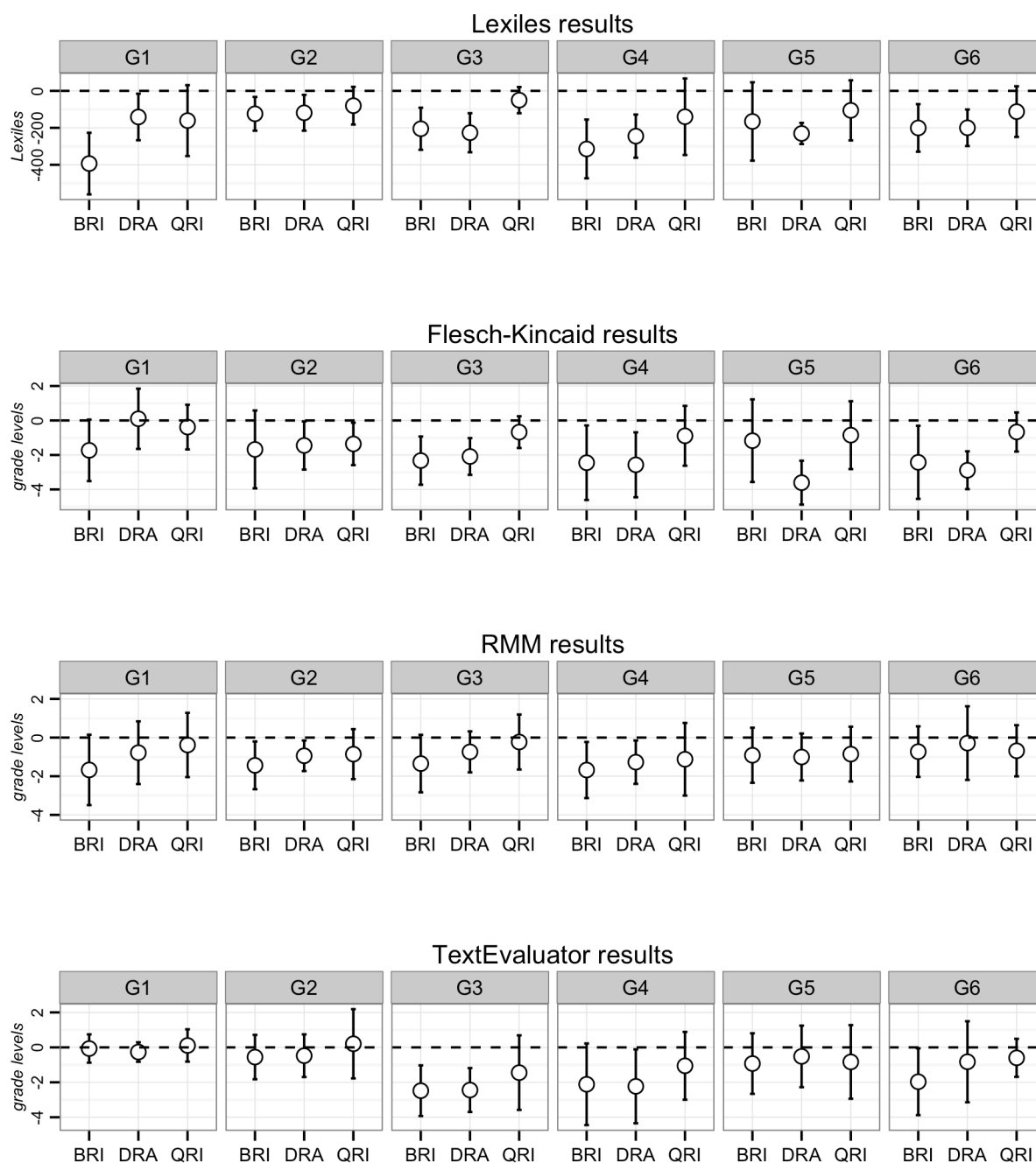
Figure 9. Estimated differences in mean complexity between DIBELS and a comparison assessment with 95% confidence intervals (constructed with Sidak corrections). The significant differences are those for which the intervals do not intersect with the dashed zero line. Lexile and Flesch-Kincaid results have more instances of significant difference (11 and 9 out of 18 comparisons respectively) than results from RMM and TextEvaluator (each shows four instances).
