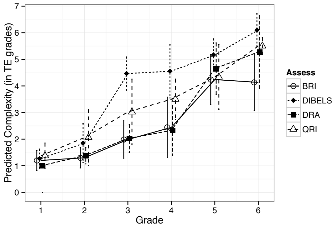
Figure 8. Grade- and assessment-specific means with 95% confidence intervals from a regression analysis, using TextEvaluator Grade Level scores as a response variable, grades, assessments, and their interactions as predictor variables. Please see caption in Figure 2.
